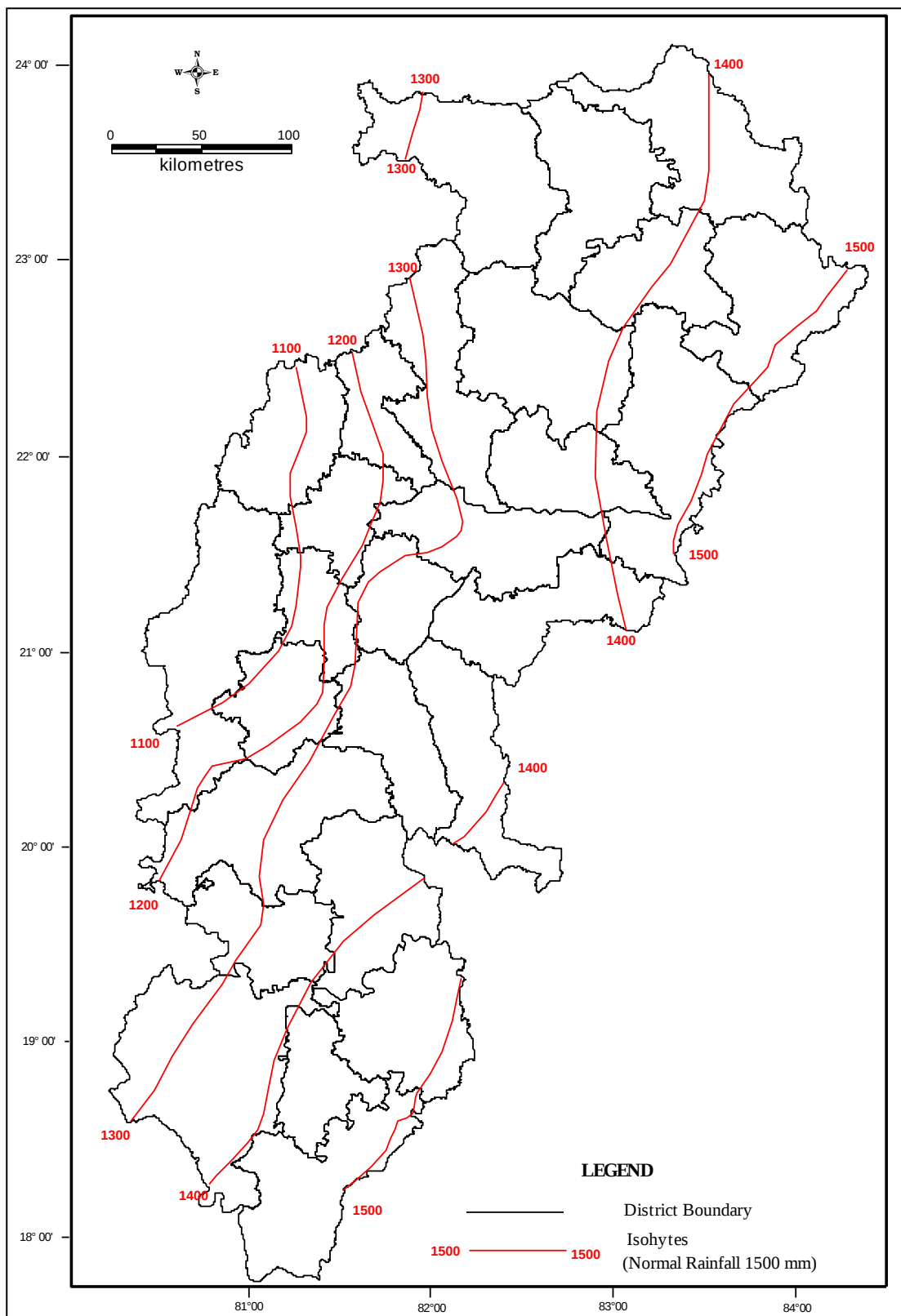
Fig 3.1: Rainfall Map of Chhattisgarh state
